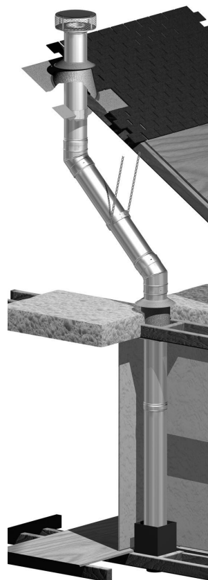
Typical Offset, Two Story Installation
