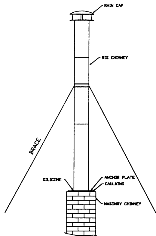
Typical Masonry Chimney Extension
