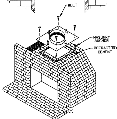
Typical Fireplace Installation
