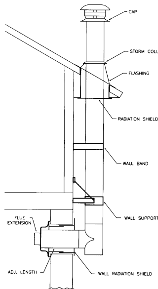
Typical Through-Wall Installation
